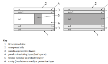
Figure 7.10 — Numbering and function of the layers in the assembly
