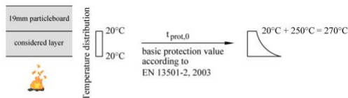
Figure 5.4. Definition of the basic protection value t_{prot,0} according to EN 13501-2.
